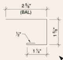
J TRIM TYPE 2 #707 (6" GIRTH)
