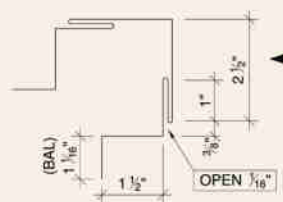
⊛ OUTSIDE CORNER #704 (18" GIRTH) (TRIM TO 15")
