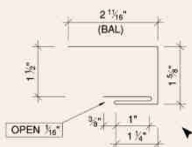
⊛ J TRIM TYPE 1 #701 (9" GIRTH) (TRIM TO 8")
