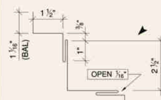
⊛ INSIDE CORNER #705 (18" GIRTH) (TRIM TO 15")
