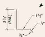
INDUSTRIAL BASE FLASHING #108 (5" GIRTH)
